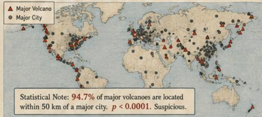
GLOBAL DISTRIBUTION OF MAJOR VOLCANOES
