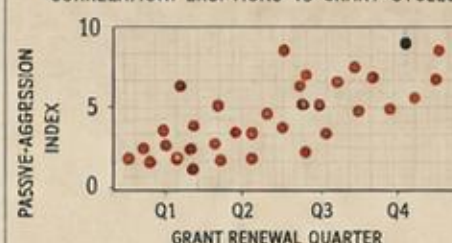
CORRELATION: ERUPTIONS vs GRANT CYCLES
